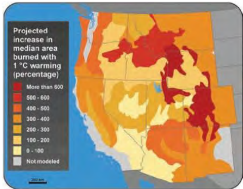
Figure 0.3. Modeled estimates of the percentage increase in area burned in the western United States (relative to 1950–2003) with a one degree increase in temperature (Peterson and Littell 2012). This projection is likely a worst case scenario as certain negative feedbacks (such as moisture dynamics) were not factored in (Don McKenzie, personal communication).
