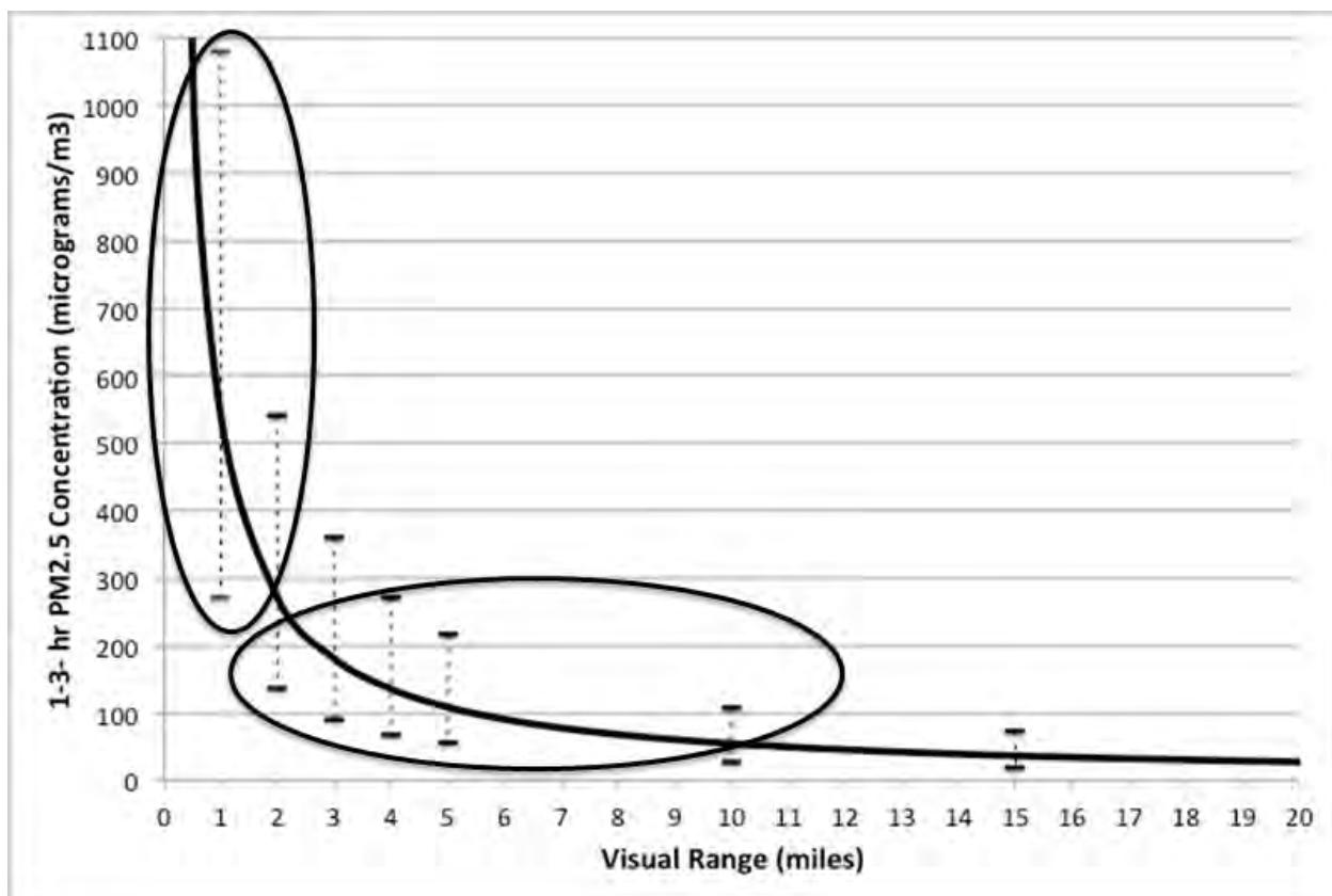
Figure 5.4.8. Relationship of visual range to PM_{2.5} concentration (adapted from Malm and Schichtel 2013). Vertical lines indicate uncertainty is especially significant when visual range is low and PM_{2.5} concentration is high. Ovals indicate broad categories of visual range such as very smoky and moderately smoky.
