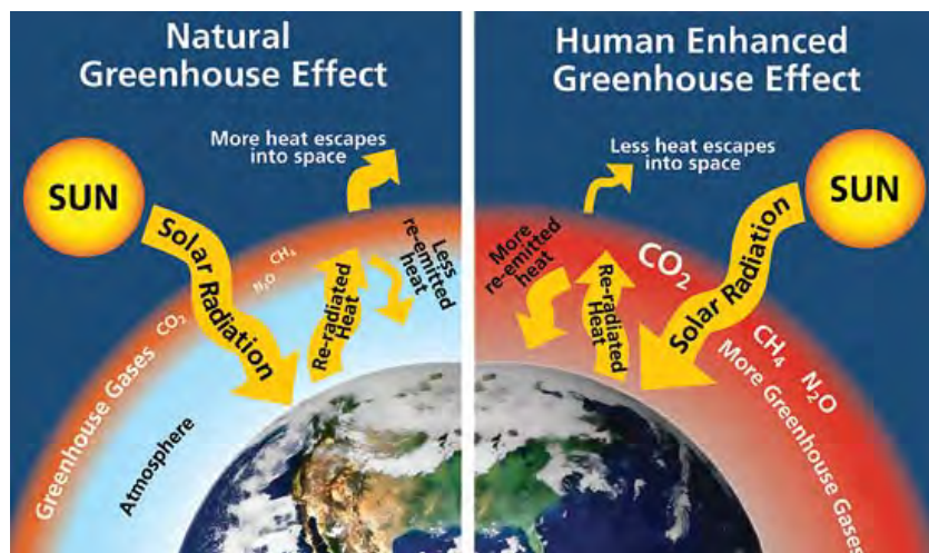
Figure 0.1. The accumulation of greenhouse gases in Earth’s atmosphere results in increased capture of heat and warms the planet. (USDI NPS 2015)
