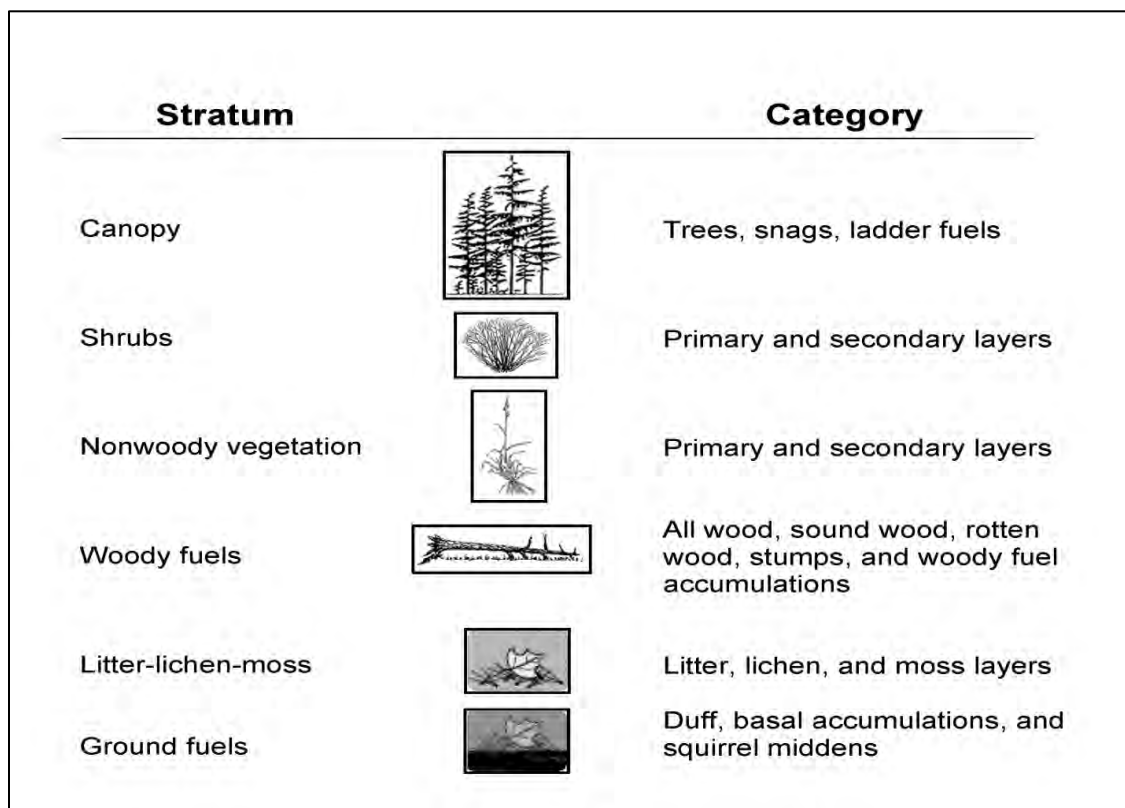
Figure 4.1.6. Stratification of a fuelbed.
