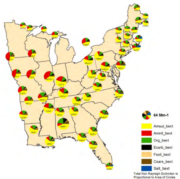
Figure 2.4.5. Annual mean composition of haze at IMPROVE sites in the Eastern United States. Most smoke effects would fall under the green “Org_bext” fraction which is an abbreviation for “organic extinction”.
