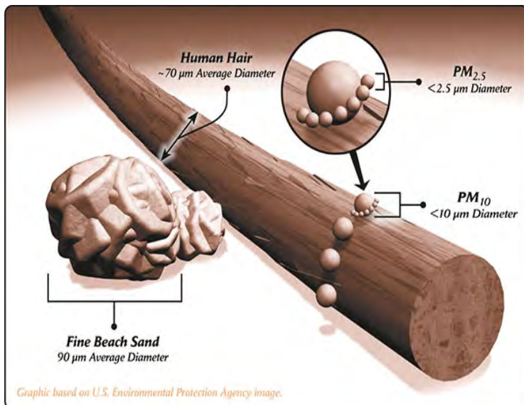
Figure 4.1.10. Relative size of PM 10 and PM 2.5 smoke particle relative to a human hair.
