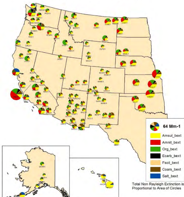
Figure 2.4.4. Annual mean composition of haze at IMPROVE sites in the Western United States. Most smoke effects would fall under the green “Org_bext” fraction which is an abbreviation for “organic extinction”.
