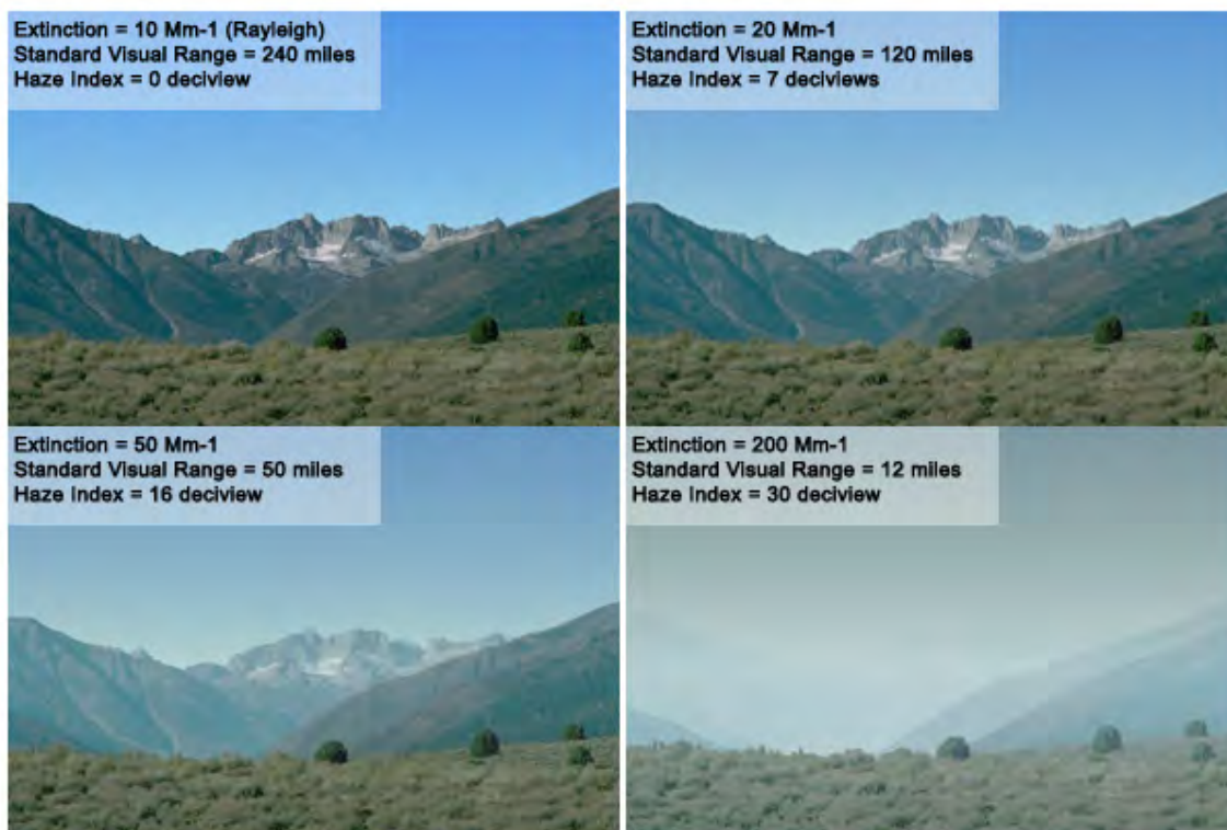
Figure 2.4.1. Computer-simulated haze at Hoover Wilderness in California. “Rayleigh scattering” is natural light scattering by the gases in the atmosphere.
