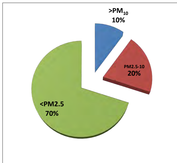
Figure 4.1.9. Particulate matter size-class distribution from typical wildland fire smoke.
